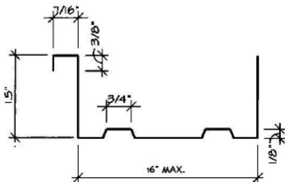
Standing Seam Panel Dimensions
