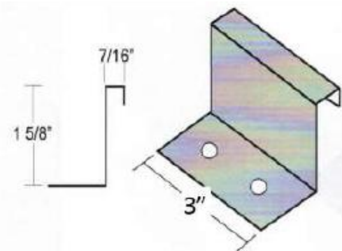
CMF1530716G24 Clip CMF1530716S24 Clip
